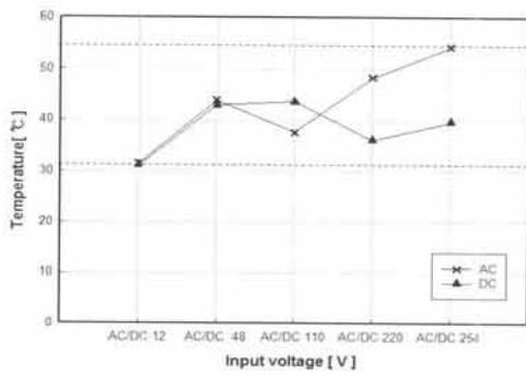
Fig. 5. Ex LED signal lamp temperature characteristics.
