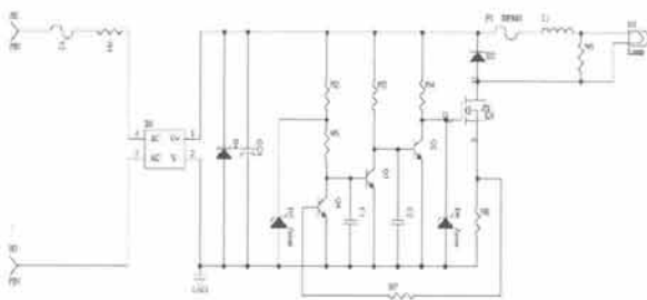
Fig. 1. Schematic of the Ex LED signal lamp.
