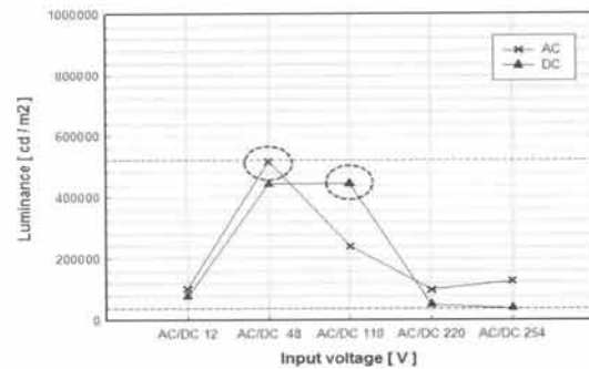
Fig. 4. Ex LED signal lamp luminance characteristics.
