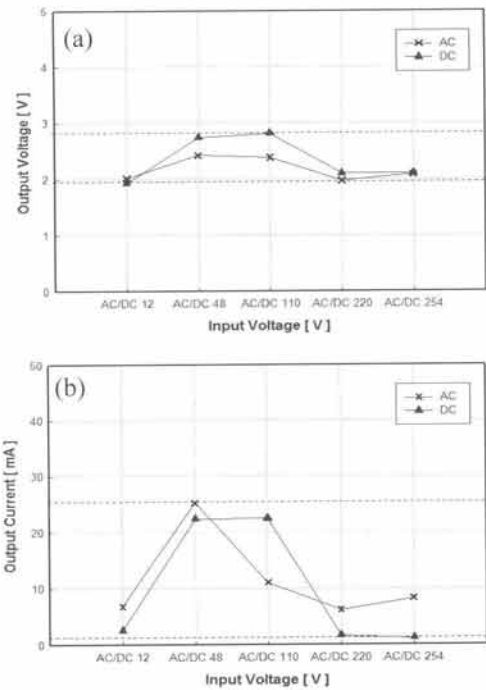
Fig. 3. AC/DC input voltage at the output. (a) output voltage and (b) output current.
