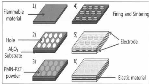
Fig. 1. Process schematic diagram for device.
