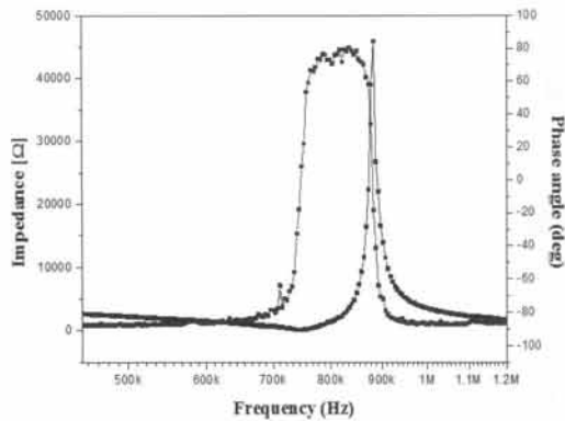
Fig. 4. Impedance and phase angle of PMN-PZT.
