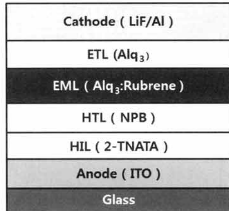
Fig. 1. Structure of fluorescent OLED.
