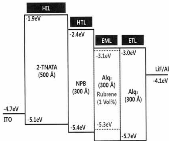
Fig. 8. Energy band diagram of fluorescent OLED.
