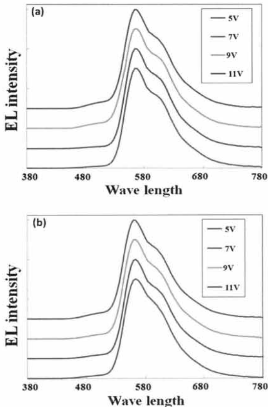
Fig. 7. EL spectra of fluorescent OLED with (a) DC power source, and (b) AC power source.
