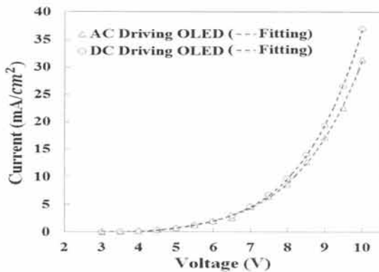
Fig. 4. Current density vs. applied voltage characteristics of fluorescent OLED with AC and DC power source.
