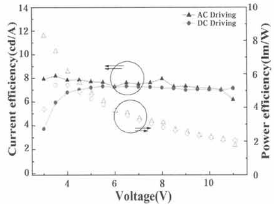
Fig. 6. Efficiency vs. applied voltage characteristics of fluorescent OLED with AC and DC power source.
