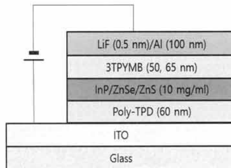
Fig. 1. Device structure of fabricated QD-LED with a InP/ZnSe/ZnS QD emission layer.
