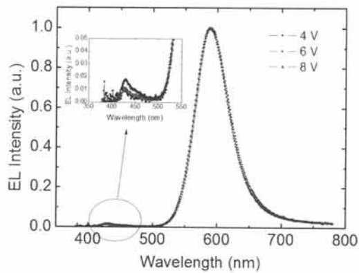
Fig. 3. EL spectra measured at several voltages for the QD-LED with a 65 nm 3TPYMB layer.
