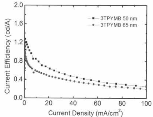
Fig. 4. Current efficiency curves as a function of current density for the QD-LEDs with 50 and 65 nm thick 3TPYMB layers.
