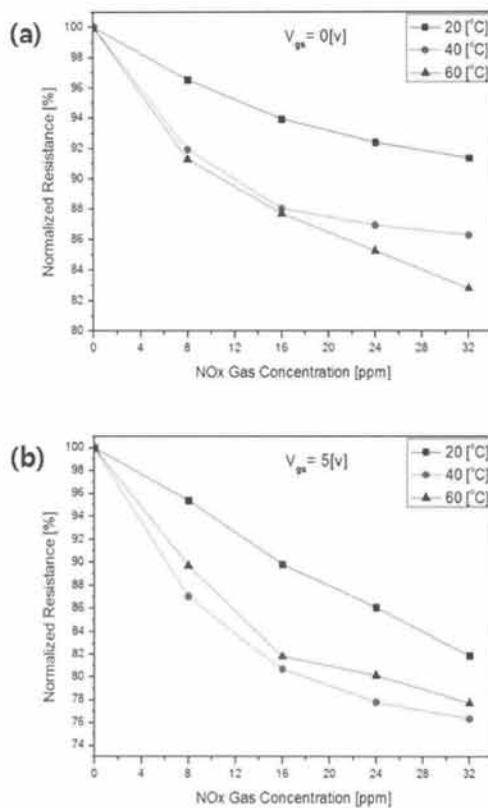
Fig. 3. The MWCNT sensor resistance change was caused by gas concentration. (a) V_{gs} = 0[V] , (b) V_{gs} = 5[V] .
