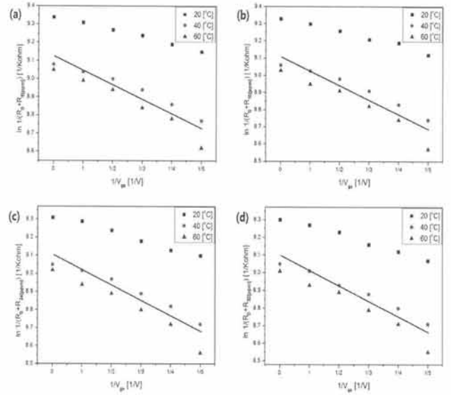
Fig. 5. The Arrhenius plot for the V_{gs} change of MWCNT films. NOx gas concentration: (a) 8[ppm], (b) 16[ppm], (c) 24[ppm], and (d) 32[ppm].
