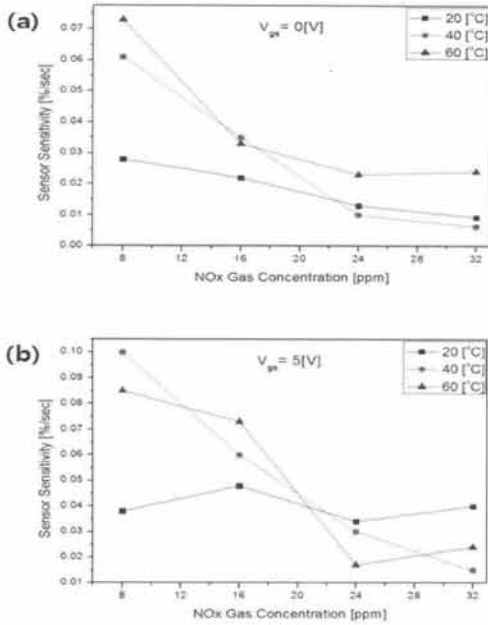
Fig. 4. Gas detection sensitivity of MWCNT gas sensor with the NOx gas. (a) V_{gs} = 0[V] , (b) V_{gs} = 5[V] .
