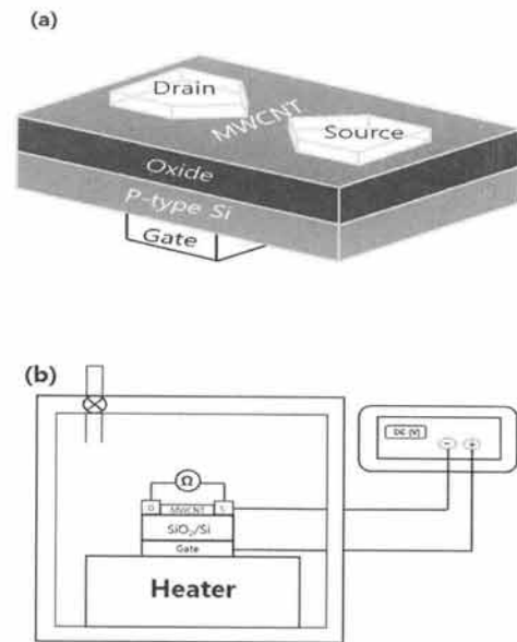
Fig. 1. (a) Schematic structure of a gas sensor, (b) Gas sensor measurement system.
