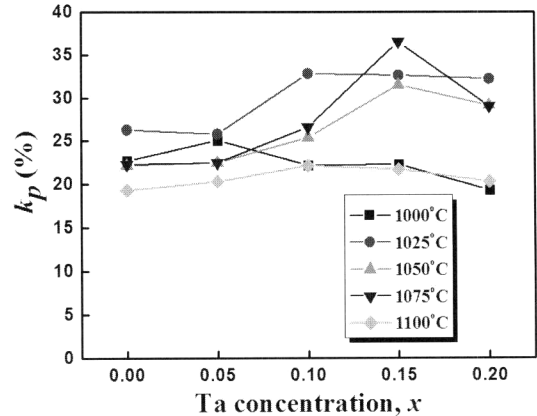
Fig. 4. Planar mode piezoelectric coupling coefficient ( k_p ) of (K_{0.5}Na_{0.5})(Nb_{1-x}Ta_x)O_3 ceramics as a function of sintering temperature.
