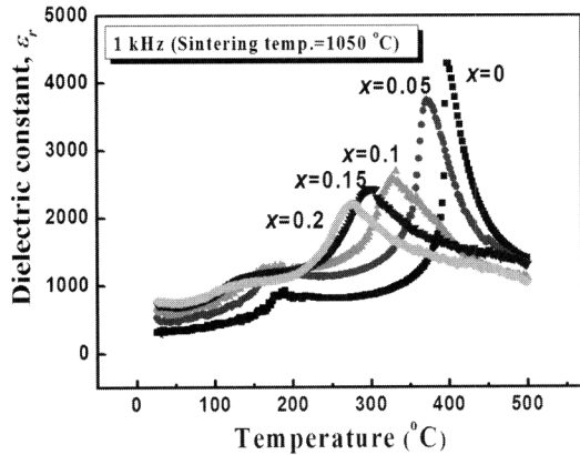
Fig. 3. Temperature dependent dielectric constant for (K_{0.5}Na_{0.5})(Nb_{1-x}Ta_x)O_3 ceramics.
