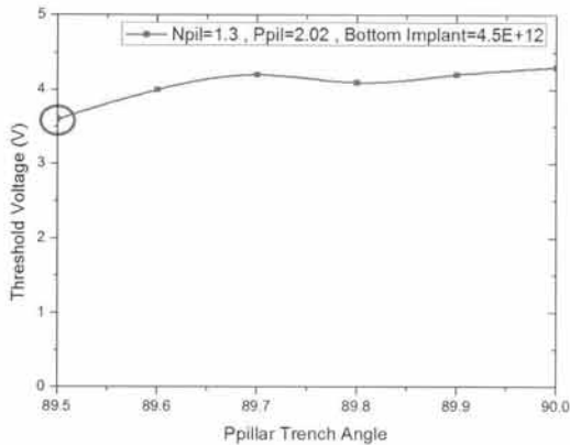
Fig. 5. The threshold voltage of SJ MOSFET according to p-pillar trench angle.
