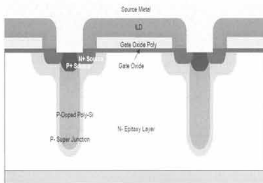
Fig. 1. The Structure of SJ MOSFET for experiments.
