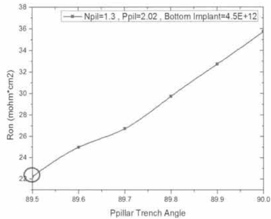
Fig. 4. The on state resistance of SJ MOSFET according to p-pillar trench angle.
