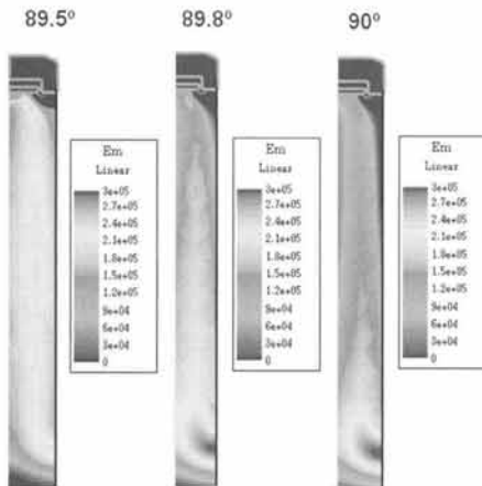
Fig. 6. The variation of depletion layer of SJ MOSFET according to p-pillar trench angle.
