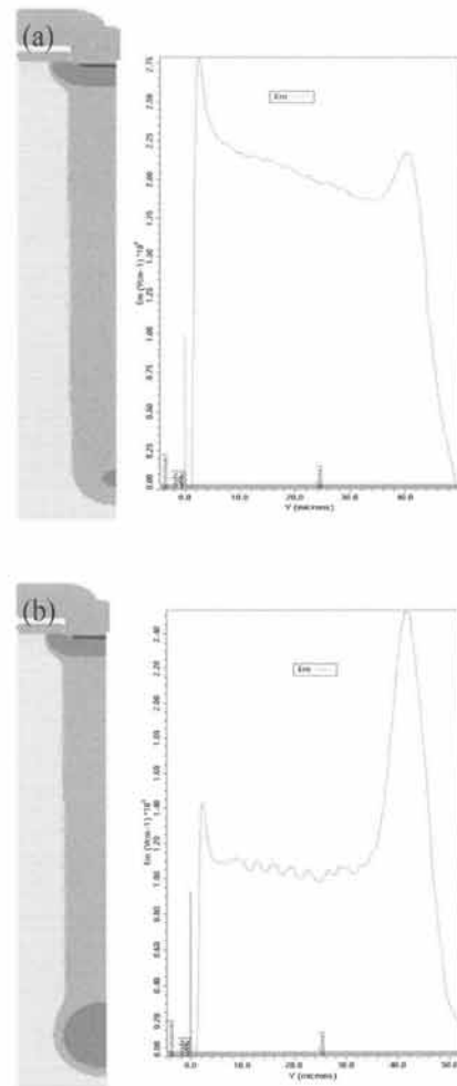
Fig. 2. Electrical distribution after process simulation of SJ MOSFET (a) not p+ boron implantation and (b) p+boron implantation.
