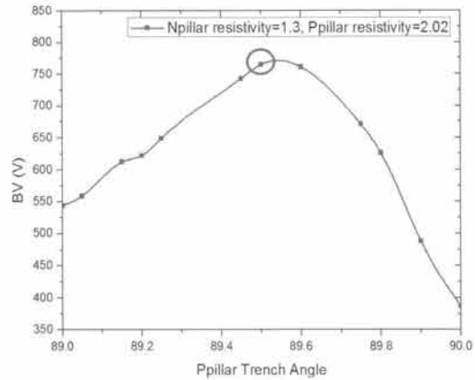
Fig. 3. The breakdown voltage of SJ MOSFET according to p-pillar trench angle.
