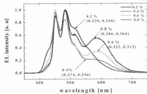
Fig. 5. EL spectra of the device.
