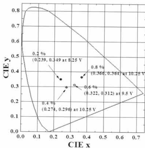
Fig. 6. CIE coordinates of the device.
