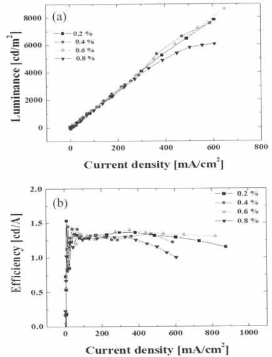
Fig. 4. (a) luminance-current density characteristics, (b) efficiency-current density characteristics.
