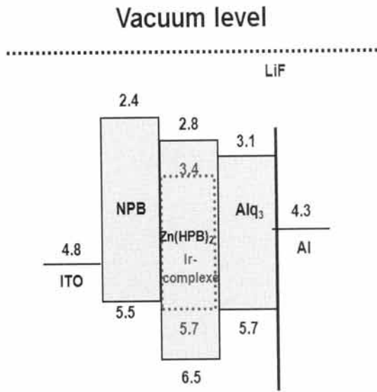
Fig. 3. The energy level alignment of the devices.
