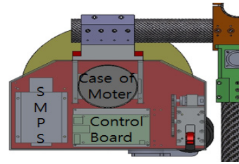
Fig. 3. Design of driving roller.
