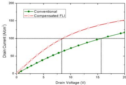
Fig. 8. Switch-on state voltage drop of conventional and compensated FLI MOSFET.
