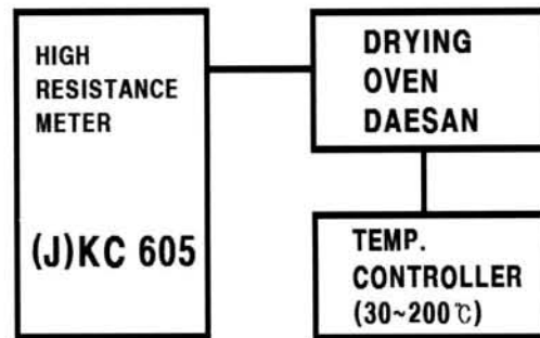
Fig. 1. Measuring circuit.
