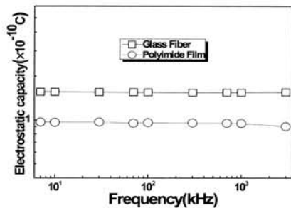
Fig. 4. Temperature dependence of C-F of thermal conductive silicone added glass fiber and polyimide film at 170°C.
