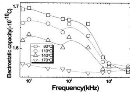
Fig. 6. Temperature degradation properties due to C vs Frequency of thermal conductive silicone rubber added glass fiber.
