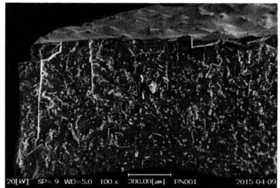
Fig. 6. Cross section of molten salt impregnated electrolyte (ZYF-50 @550°C).
