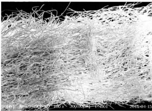
Fig. 4. Cross section of ceramic felt (ZYF-50).
