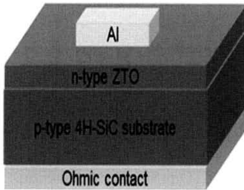
Fig. 1. Schematic illustration of a n-ZTO/p-4H-SiC heterojunction device.
