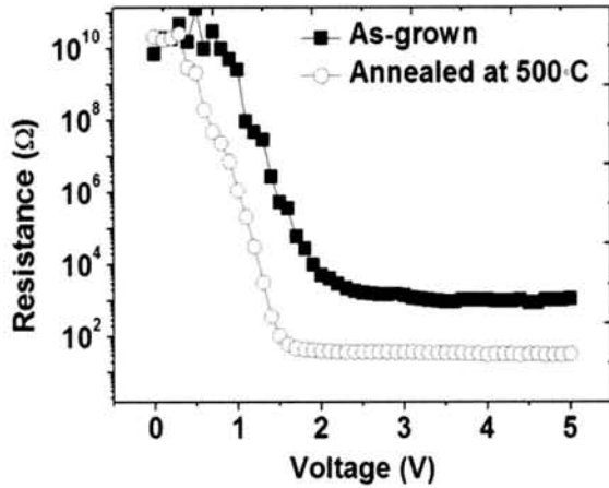
Fig. 3. Resistance ( dV/dI ) versus voltage for the n-ZTO/ p-SiC heterojunction diode fabricated on as-grown, annealed at 500°C.
