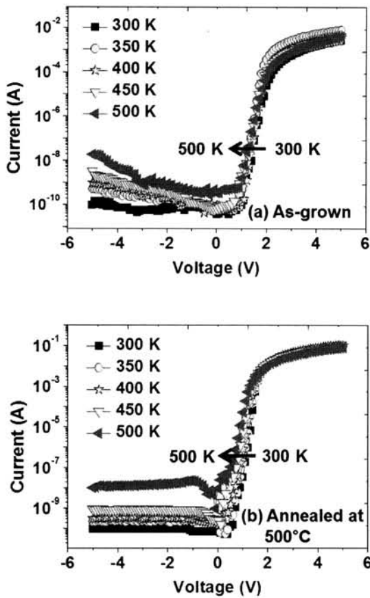
Fig. 5. I-V semi-logarithm curves of ZTO/4H-SiC hetero-junction as a function of temperature from 300 K to 500 K; (a) as-grown and (b) annealed at 500°C.
