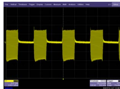
Fig. 1. Waveform of inverter surge.
