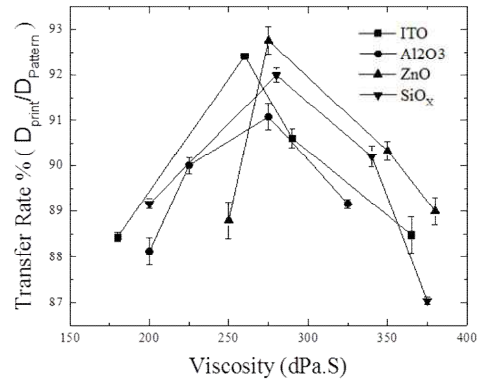
Fig. 4. The variation of transfer rate along with the paste viscosity.
