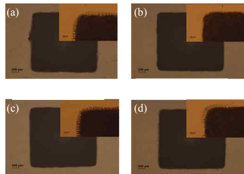
Fig. 3. The variation of screen printed pattern shape depending on the paste viscosity. (a) 180 dPa·s, (b) 260 dPa·s, (c) 290 dPa·s, and (d) 365 dPa·s.
