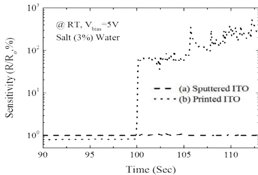
Fig. 6. Comparison of sensing properties of sputtered and printed ITO layers.
