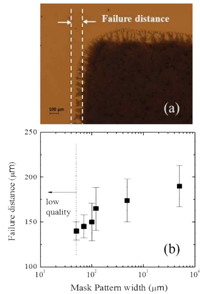
Fig. 2. (a) Printed ITO pattern image, (b) various failure distance of printed ITO pattern dependence on mask pattern width.
