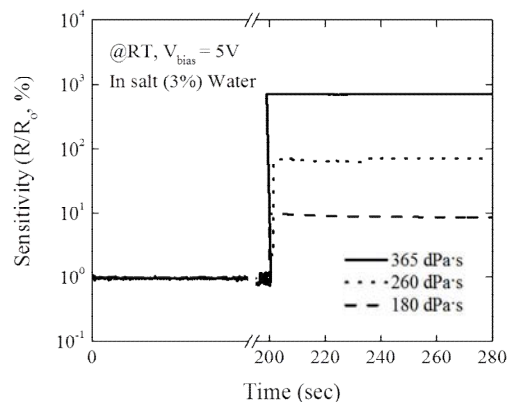
Fig. 5. Liquid sensing properties of printed ITO sensor.
