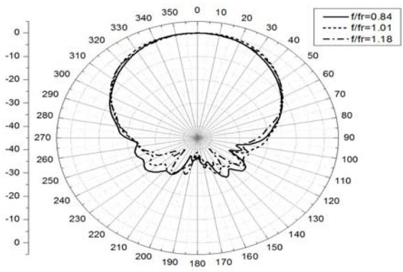
Fig. 11. Measured beam patterns of piezoelectric single crystal Tonpizl transducer.
