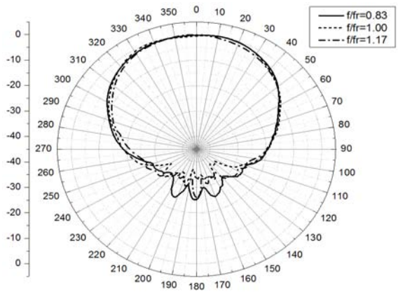
Fig. 10. Measured beam patterns of piezoelectric ceramic Tonpizl transducer.
