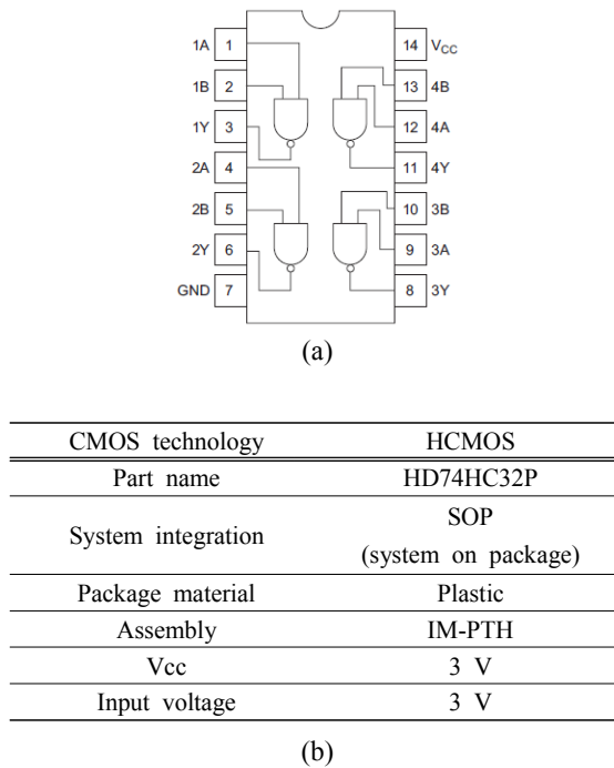
Fig. 4. DUT specification. (a) IC pin arrangement and (b) OR gate IC specification.
