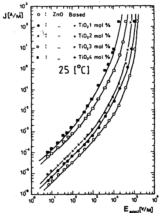
Fig. 5 Effects of TiO_2 contents on the V-I characteristics of ZnO varistor.
