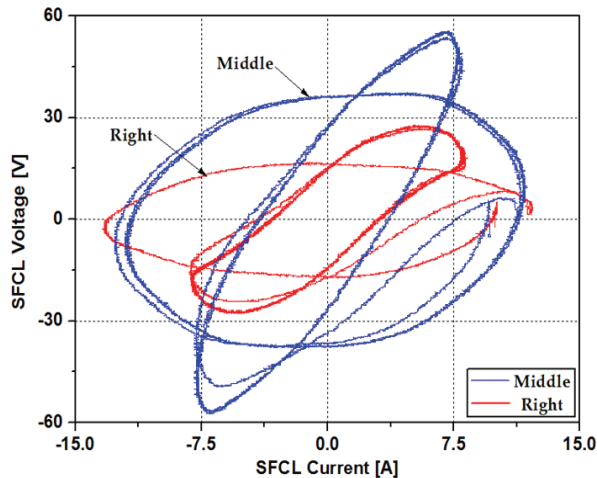
Fig. 9. V_{SFCL} - I_{SFCL} curve during fault.
