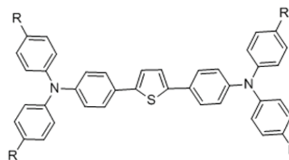
Fig. 1. Thiophene-amine structure.
