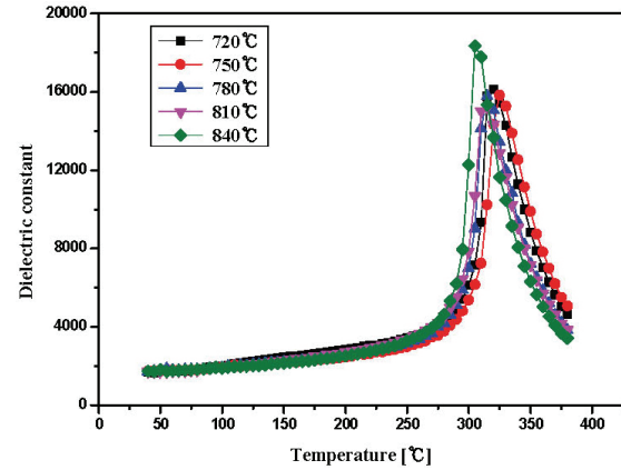
Fig. 7. Temperature dependence of dielectric constant and the Curie temperature ( T_c ) with 2nd calcination temperature.
