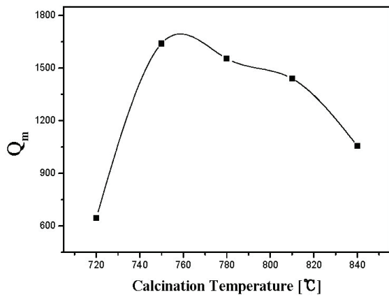
Fig. 5. Electrotechnic quality factor ( Q_m ) of specimens with 2nd calcination temperature.
