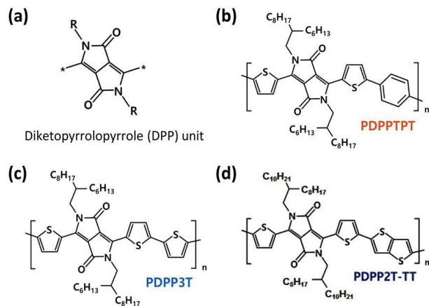
Fig. 1. Molecular structure of (a) diketopyrrolopyrrole (DPP) unit, (b) PDPPTPT, (c) PDPP3T, and (d) PDPP2T-TT.
