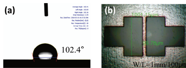
Fig. 2. (a) Deionized water contact angle of ODTS-treated SiO 2 surface and (b) shadow mask for S/D electrodes (with channel width/length=1 mm/100 μm).
