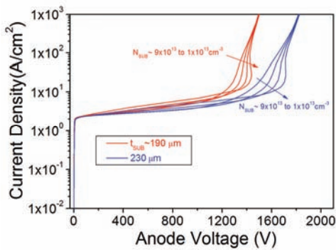
Fig. 4. Breakdown characteristics of SITHs for different substrate thickness and doping concentration values.
