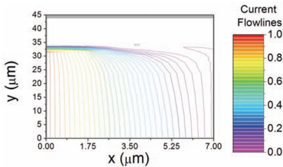
Fig. 3. Current flow lines at device break down of SITH.
