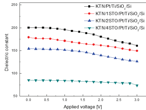
Fig. 4. Dielectric constant of KTN/STO thin films with the number of STO coatings and applied voltage.
