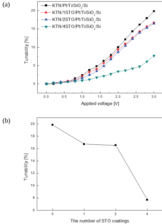
Fig. 5. Tunability of KTN/STO thin films with (a) applied voltage and (b) the number of STO coatings at 3 V, respectively.
