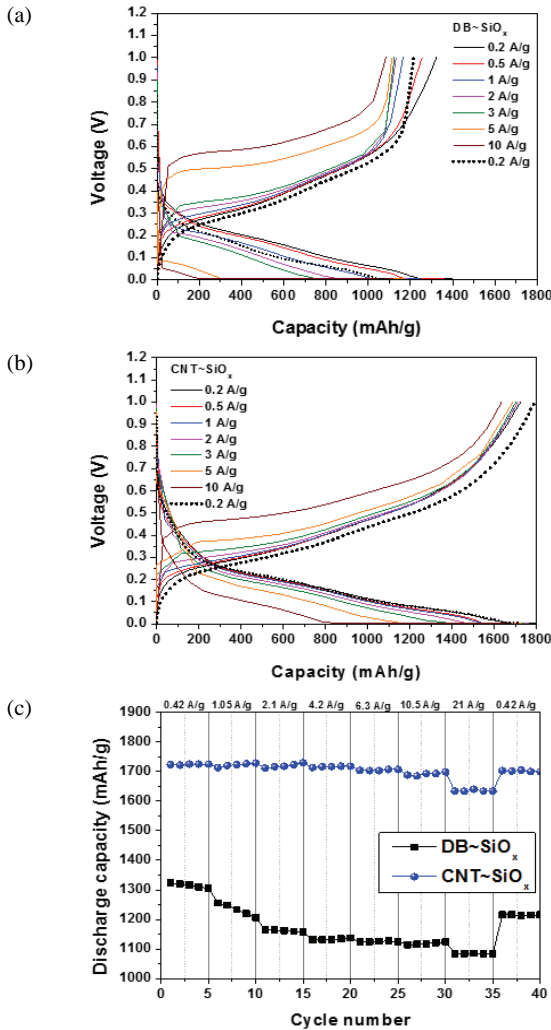
Fig. 6. Charge-discharge profiles of SiOx with (a) DB (b) CNT conductive agents at various current densities, and (c) rate capability of SiOx with DB or CNT conductive agents.
