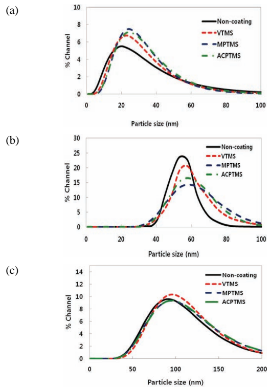
Fig. 3. Particle size distributions of hybrid sol with various surface treatment agent. (a) Particle size of silica: 20 nm, (b) particle size of silica: 60 nm, and (c) particle size of silica: 90 nm.
