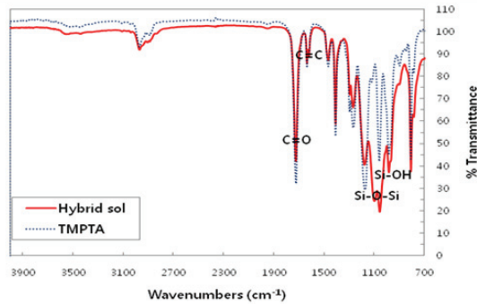
Fig. 6. FT-IR of TMPTA and hybrid sol.
