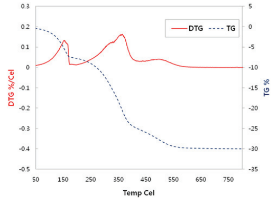
Fig. 5. TG/DTG graph of MPT2070 hybrid sol.
