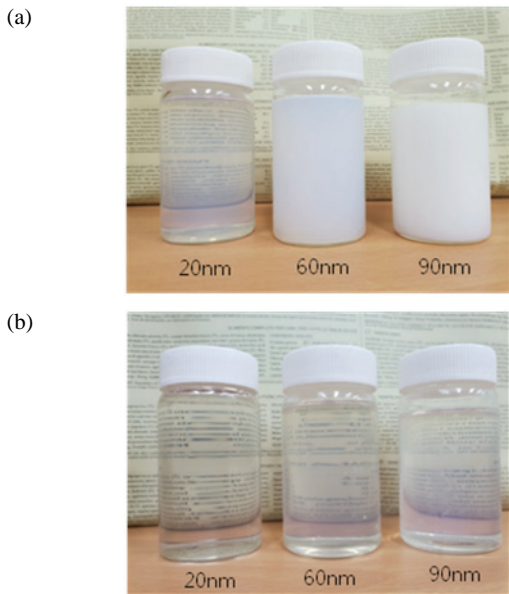
Fig. 4. Photograph of colloidal silica and hybrid sol. (a) Colloidal silica and (b) non-solvent hybrid sol.
