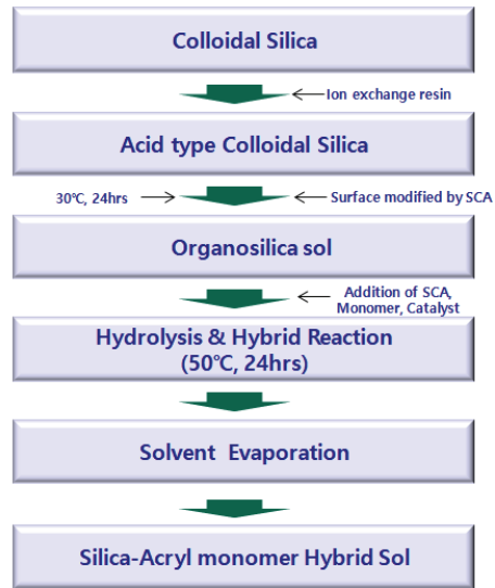
Fig. 1. Flow chart for preparation of hybrid coating sol.
