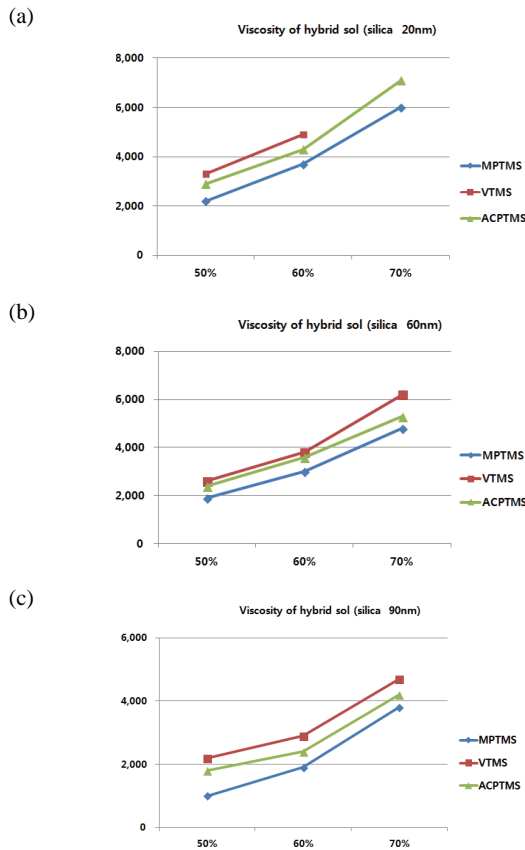
Fig. 2. Viscosities of hybrid sol as a function of particle size of silica. (a) Particle size of silica: 20 nm, (b) particle size of silica: 60 nm, and (c) particle size of silica: 90 nm.
