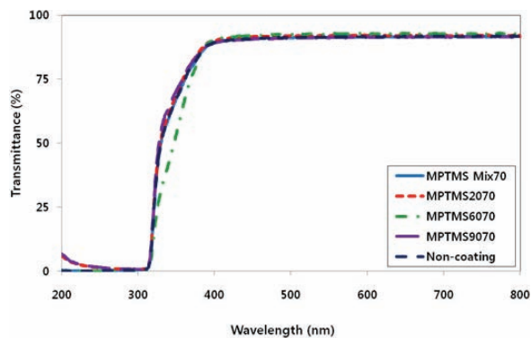
Fig. 7. Optical transmittance of silica hybrid coated on PET film in visible wavelength range.
