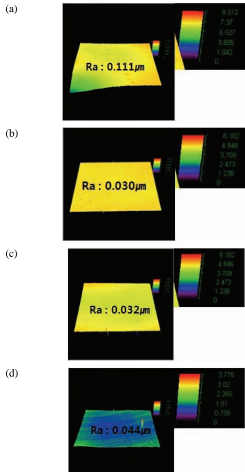
Fig. 8. 3D microscope photograph of silica hybrid coated on PET film. (a) MPTMS 2070, (b) MPTMS 6070, (c) MPTMS 9070, and (d) MPTMS-Mix 70.
