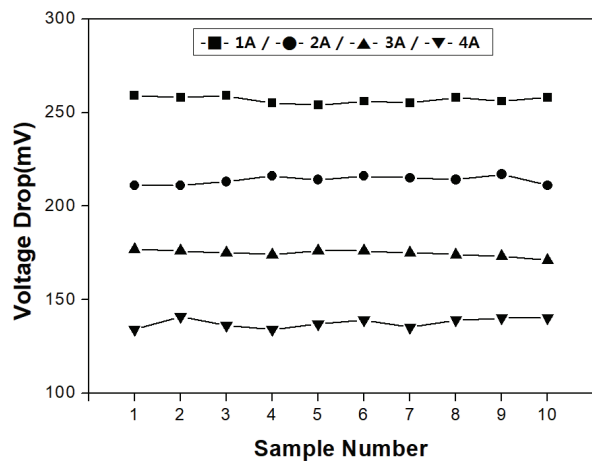
Fig. 3. Test result of voltage drop.
