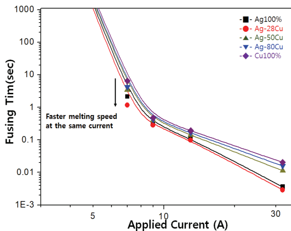
Fig. 5. Change in rated current according to the wire composition of Ag-Cu alloy.
