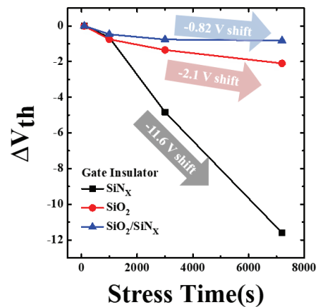
Fig. 4. The \Delta V_{th} shift of the Si_3N_4 , SiO_2 , and SiO_2/Si_3N_4 gate insulator are -11.6 V, -2.1 V and -0.82 V [20].
