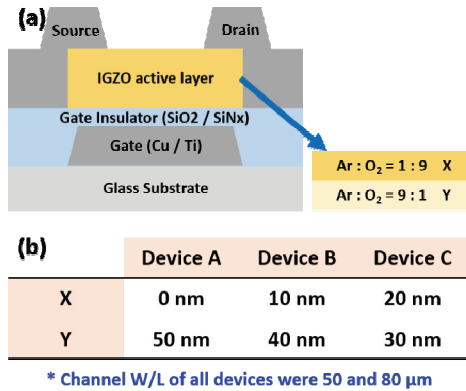
Fig. 5. (a) Schematic diagram of device with dual IGZO active layer. (b) Compare the oxygen-poor layer and oxygen-rich layer thickness of each device.
