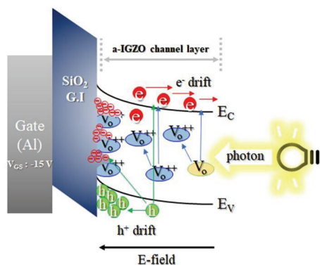
Fig. 1. Schematic energy band diagram to explain the trapping or/injection of a photo induced hole carrier.
