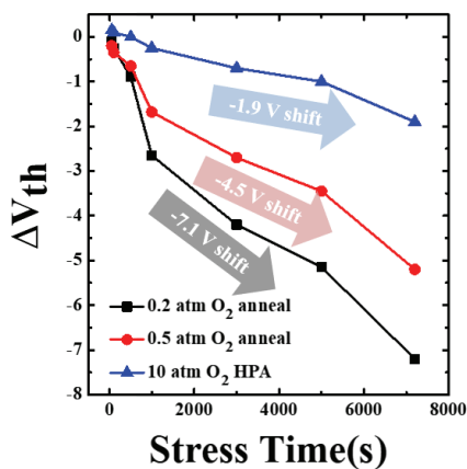
Fig. 2. Threshold voltage shift in the NBIS condition of the O_2 annealed device at different pressures. The \Delta V_{th} shift of the 0.2 atm, 0.5 atm, and 10 atm device are -7.1 V, -4.5 V and -1.9 V, respectively [13].
