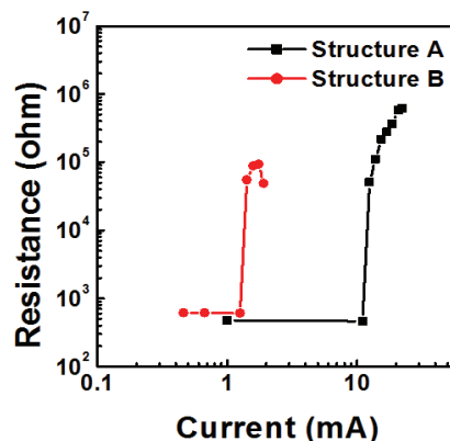
Fig. 4. Resistance vs current for chalcogenide PCM devices.
