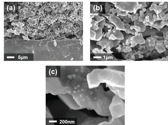
Fig. 4. (a) Microstructural observations for composite anode of \text{La}(\text{Sr})\text{Ti}(\text{Ni})\text{O}_3 - \text{Ce}(\text{Mn,Fe})\text{O}_2 after the cell operation, (b) magnified, and (c) observations of Ni exsolution on the surface of the anode.
