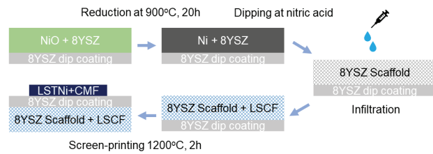
Fig. 2. Schematic diagram for preparation of cathode-supported button cell.
