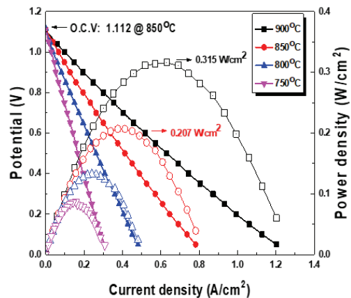
Fig. 7. Evaluation of the cell performance of the fabricated cathode-supported button cell.
