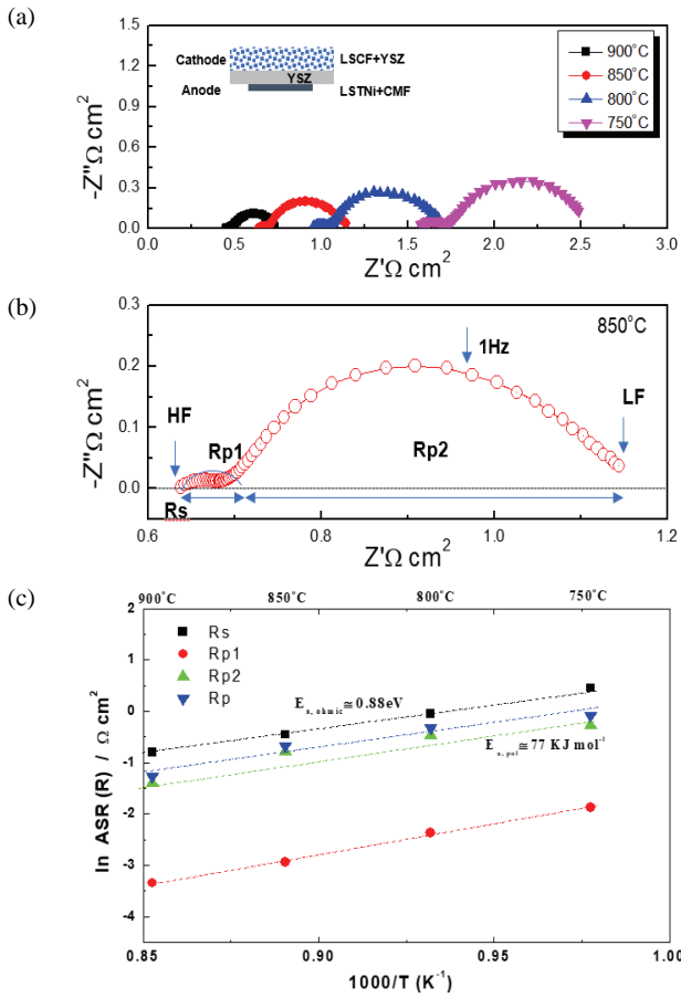
Fig. 8. (a) Impedance results of the fabricated cathode-supported button cell, (b) impedance results at 850°C; showing that polarization resistance with low frequency area accounts for the most of the impedance, and (c) activation curves calculated from impedance spectra.
