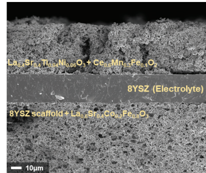
Fig. 3. SEM images of fabricated button cell.
