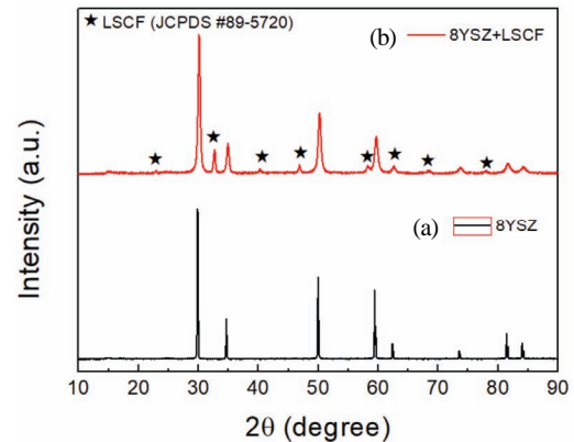
Fig. 6. XRD patterns of the cathodic side of the fabricated cathode-supported button cell; (★) marks correspond to peaks of LSCF.
