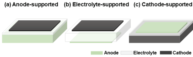
Fig. 1. Structural classification of SOFCs.
