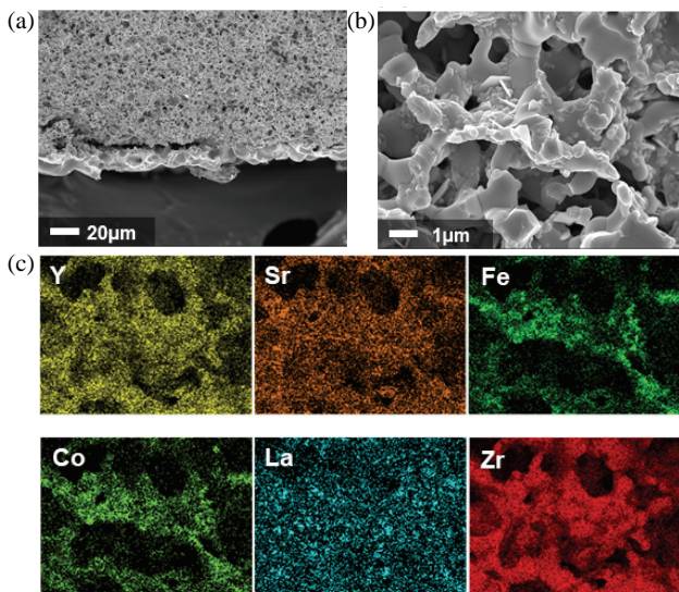
Fig. 5. (a) Microstructural observations of cathode, (b) magnified, and (c) EDX mapping results of magnified cathode microstructure.
