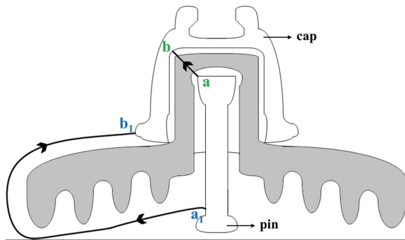
Fig. 1. Leakage paths inside and outside the insulator.
