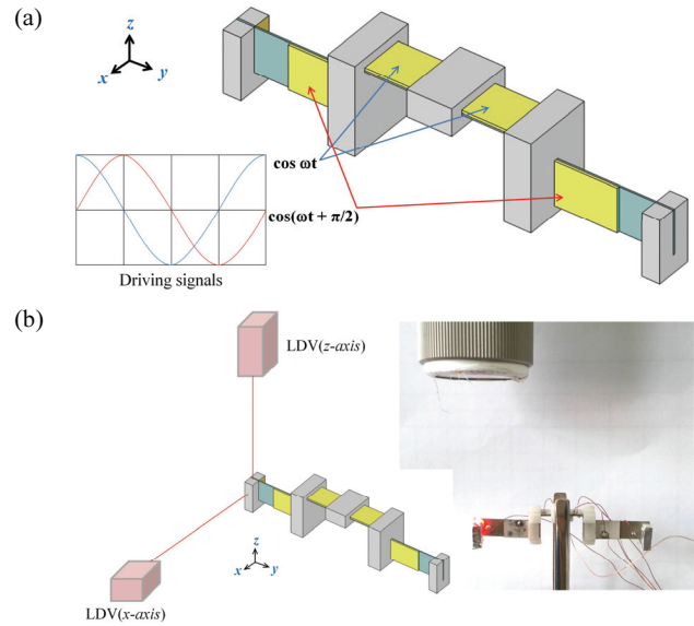
Fig. 8. (a) Input signals and (b) experimental setup and measurement of displacement at the tip of actuator.
