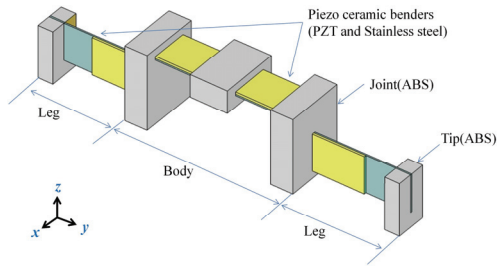
Fig. 3. Structure and materials of the actuator.
