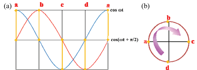
Fig. 2. Elliptical motions of actuator: (a) Driving signals and (b) elliptical motions at the tips.
