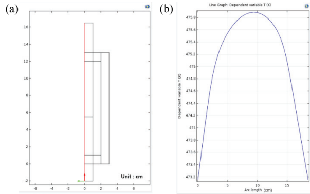
Fig. 6. Thermal distribution of VI cross section. (a) Cross section and (b) thermal distribution.
