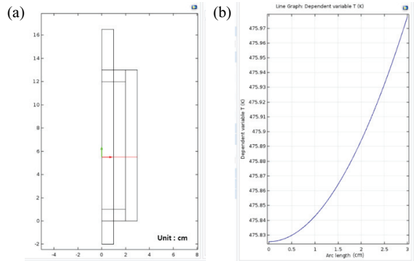
Fig. 7. Thermal distribution of VI cross section. (a) Cross section and (b) thermal distribution.
