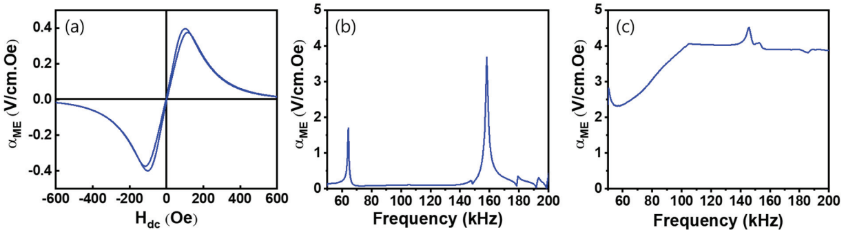
Fig. 5. ME voltage coefficient, \alpha_{ME} for 31-Ni ME composite, (a) off-resonance magnetolectric voltage coefficient, \alpha_{ME} , of Rosen type piezoelectric transducer under an H_{dc} of 1 Oe at 1 kHz, (b) frequency dependency of \alpha_{ME} , from V_{a1} at 0 Oe, and (c) frequency dependency of \alpha_{ME} , from V_{a2} at 101 Oe bias field.
