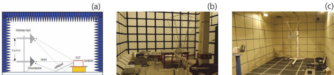
Fig. 3. Composition photo of the experimental device. (a) Anechoic chamber, (b) EMI TEST for anechoic chamber, and (c) EMS test for anechoic chamber.
