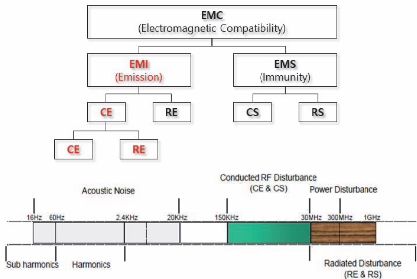
Fig. 1. Electromagnetic compatibility.
