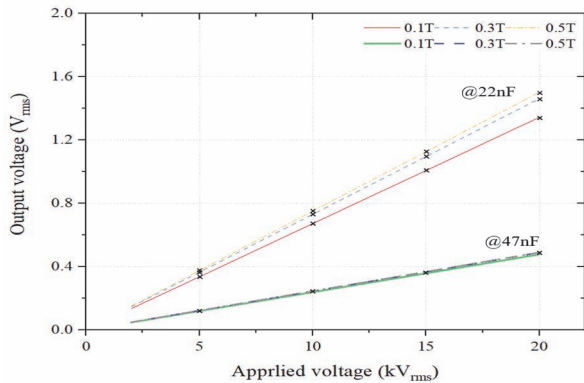
Fig. 4. Comparison of voltage ratio.
