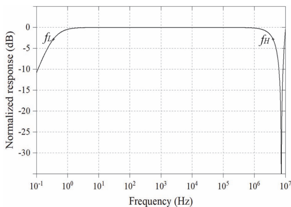
Fig. 5. Frequency response of the capacitive probe.
