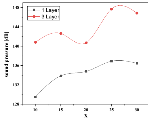
Fig. 7. Sound pressure of ultrasonic cleaner with the dimension of ceramics.
