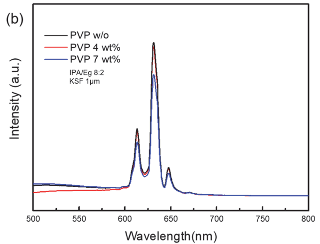
Fig. 7. (a) Dispersion characteristics of KSF phosphor inks according to PVP content and (b) PL intensity of KSF phosphor inks.
