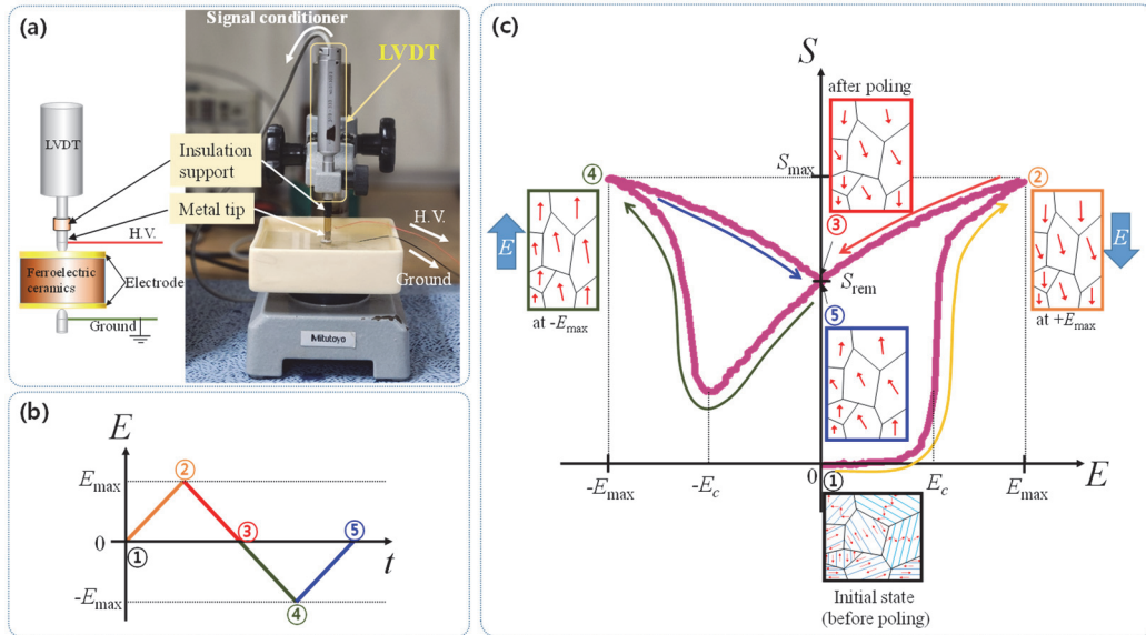
Fig. 4. Example of measurement of field-induced-strain characteristics of ferroelectric ceramics using LVDT: (a) schematic diagram and photo of the measurement system, (b) input signal for measuring field-induced-strain characteristics of ferroelectric ceramics, and (c) virgin strain curve of \text{Bi}_{1/2}(\text{Na}_{0.82}\text{K}_{0.18})_{1/2}\text{TiO}_3 (BNKT18) ceramics and schematic diagram of ferroelectric domain state changes.
