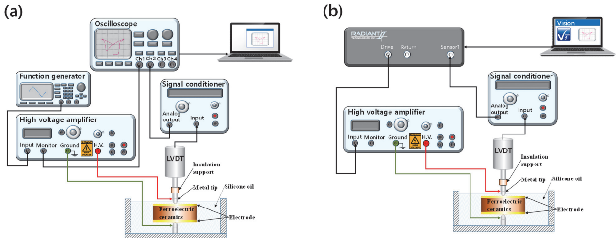
Fig. 3. Schematic figure of the experimental setup for electric-field-induced strain measurement of ferroelectric ceramics using a LVDT: (a) a system consisting of a function generator, high voltage amplifier, LVDT, signal conditioner and oscilloscope and (b) a system consisting of RADIANT's ferroelectric tester, high voltage amplifier, LVDT, and signal conditioner.
