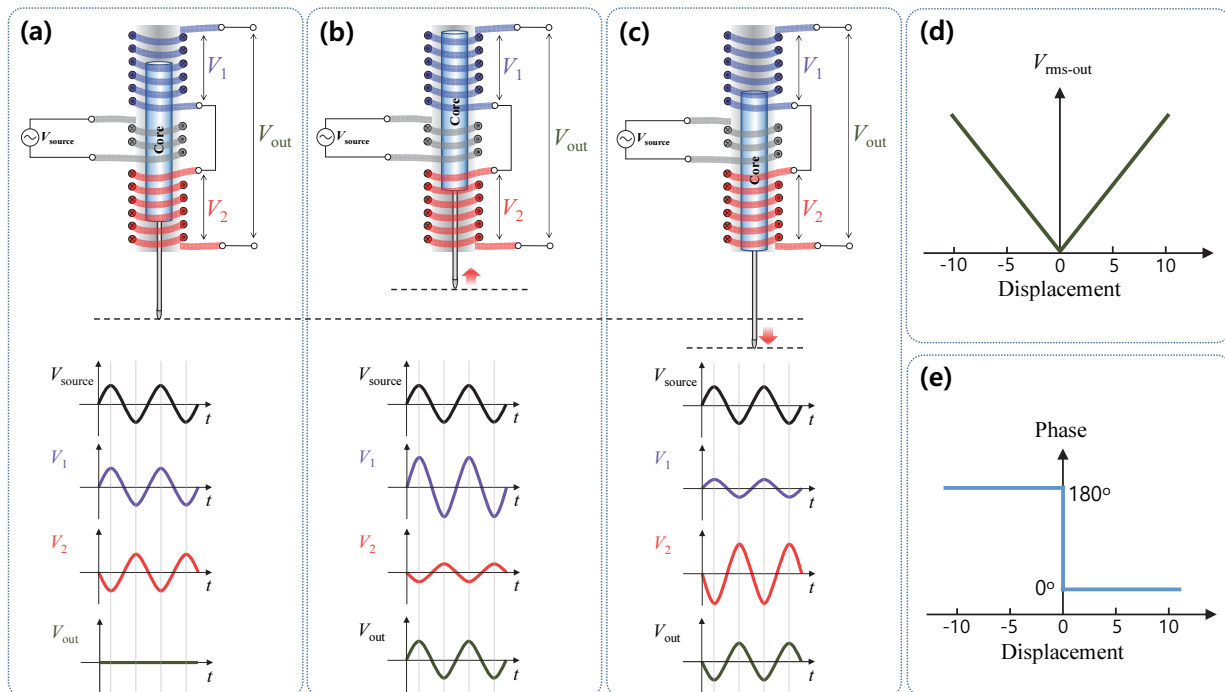
Fig. 2. Schematic diagram of the operating principle of an LVDT sensor: schematic diagram of the movement of the core in the LVDT and the signals of V_{source} , V_1 , V_2 , and V_{out} when the displacement is (a) 0, (b) positive, and (c) negative, (d) change in output V_{rms} value and (e) phase difference between V_{source} and V_{out} signals according to displacement.
