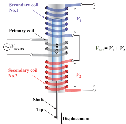
Fig. 1. Structure illustration of linear variable differential transducer (LVDT).
