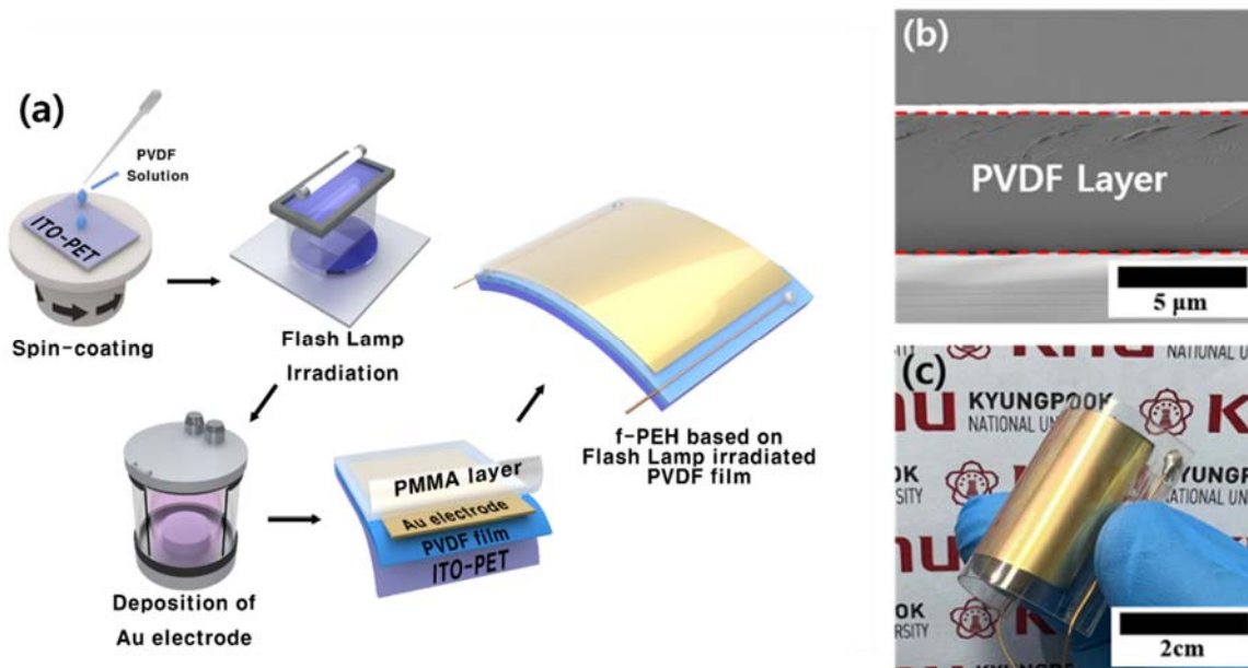
Fig. 3. (a) Schematic illustrations showing the fabrication process of the flexible piezoelectric energy harvester based on flash lamp irradiated PVDF films, (b) cross-sectional SEM image of the piezoelectric PVDF layer, and (c) photograph of the fabricated flexible piezoelectric energy harvester with a size of 3 \times 4 \text{ cm}^2 .
