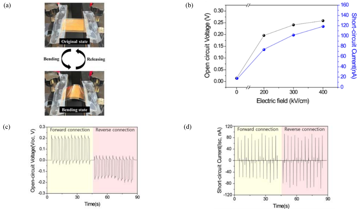
Fig. 4. (a) Photographs of the flexible piezoelectric energy harvester in bending and original states, (b) open-circuit voltage and short-circuit current measured from the energy devices after poling process at 200, 300, and 400 kV/cm, and (c,d) open-circuit voltage: (c) and short-circuit current (d) measured under forward and reverse connections, respectively.
