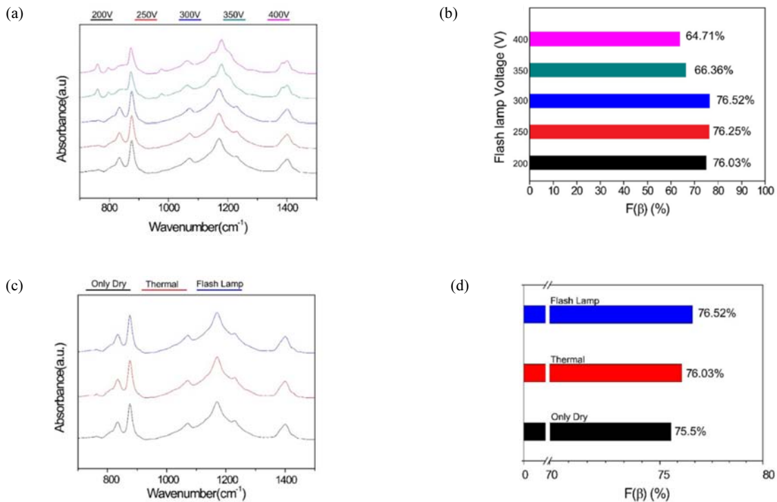
Fig. 2. (a,b) FT-IR spectra: (a) and the calculated \beta -phase fraction (b) of PVDF films irradiated with a flash lamp at 200, 250, 300, 350, and 400 V. (c) FT-IR spectra of only dried, thermal annealed, and flash lamp annealed PVDF films.
