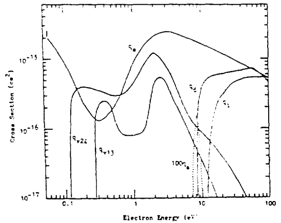
Fig. 8. The derived electron collision cross sections for SiH 4 molecules: qm-momentum transfer cross section; q v24 and q v13 -vibrational excitation cross sections; q a -attachment cross section; q d -dissociation cross section; and q i -ionization cross section.
