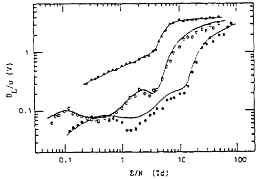
Fig. 7. The ratio of the longitudinal diffusion coefficient to the electron mobility in SiH 4 -Ar mixtures.
