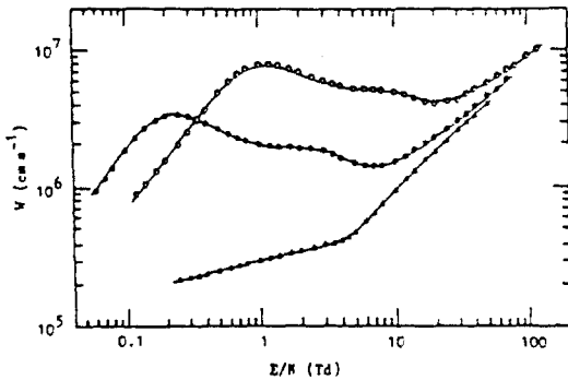
Fig. 6. The electron drift velocity in SiH 4 -Ar mixtures as a function of E/N.
